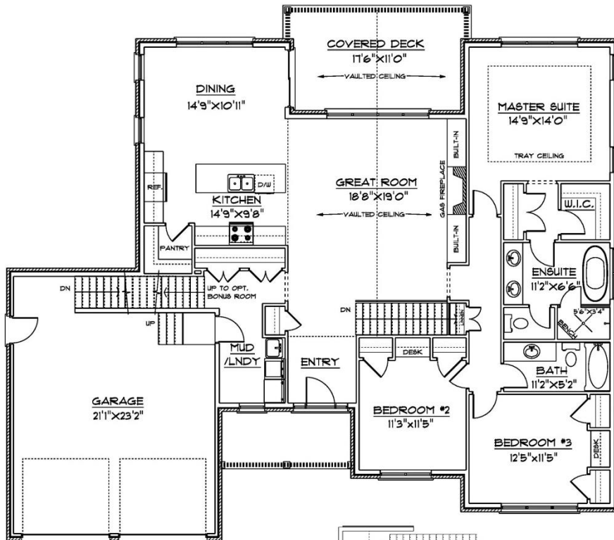
MAIN FLOOR
