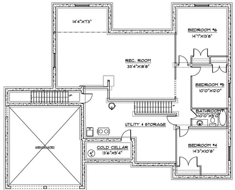
BASEMENT
